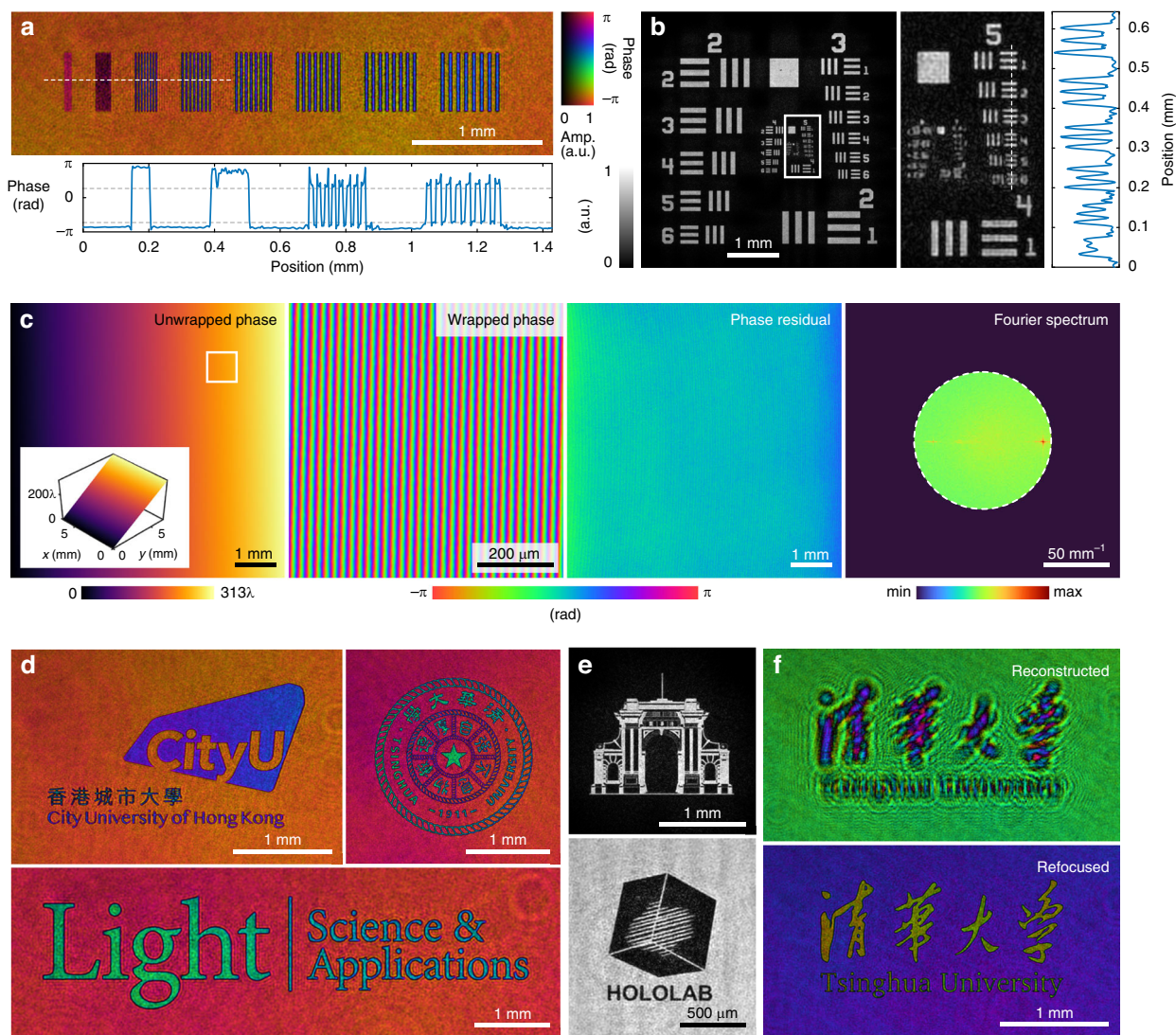
Fig. 4 Performance characterization of the wavefront sensor. a Reconstructed complex amplitude of a phase resolution pattern, where the line widths vary from 1 to 8 SLM pixels from left to right, and the finest resolvable line width is 11.22\ \mu\text{m} , corresponding to 3 SLM pixels. The cross-sectional phase profile is shown below, where the range between the two dashed lines indicates the theoretical phase retardance of \pi . Note that the reconstructed phase values of the first two groups of line patterns deviate from the theoretical values due to aliasing effects. b Reconstructed amplitude and the amplitude cross-sectional profile of a negative 1951 USAF amplitude resolution test target, where the finest resolvable line width is 8.77\ \mu\text{m} (Group 5, Element 6). c Wavefront reconstruction of a tilted plane wave. From left to right: unwrapped phase profile within a 2800 \times 2800 FOV, enlarged FOV of the wrapped phase profile corresponding to the boxed region, phase residual map compared to the reference ptychographic measurement, and Fourier modulus (in logarithmic scale) of the reconstructed wavefront, where the dashed circle indicates the support region. d Reconstructed complex amplitude of representative phase objects. e Reconstructed amplitude profiles of negative (upper) and positive (lower) amplitude objects. f Demonstration of autofocusing, where the directly reconstructed (upper) and refocused (lower) wavefronts are shown (Supplementary Video 1)
