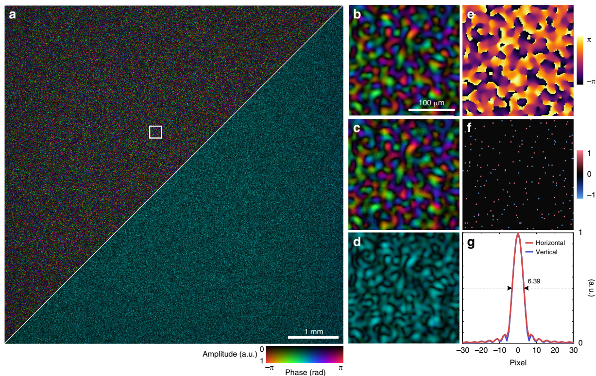
Fig. 7 Wavefront sensing application for complex speckle fields. a Full-field-of-view holographic reconstruction of a speckle field containing approximately 192,000 spatial modes (upper left) and the corresponding phase-conjugated wavefront (lower right). b–d Enlarged region of interest in (a) . Results obtained via SAFARI (b) , ptychographic measurements (c) , and the phase-conjugated wavefront (d) are shown. e Phase profile of (b) . f Calculated topological charge map reveals the phase singularities in (e) . g Horizontal and vertical cross sections of the autocorrelation of the speckle field profile in (a) . The average FWHM is 6.39 pixels, which approximately corresponds to the average speckle grain size
